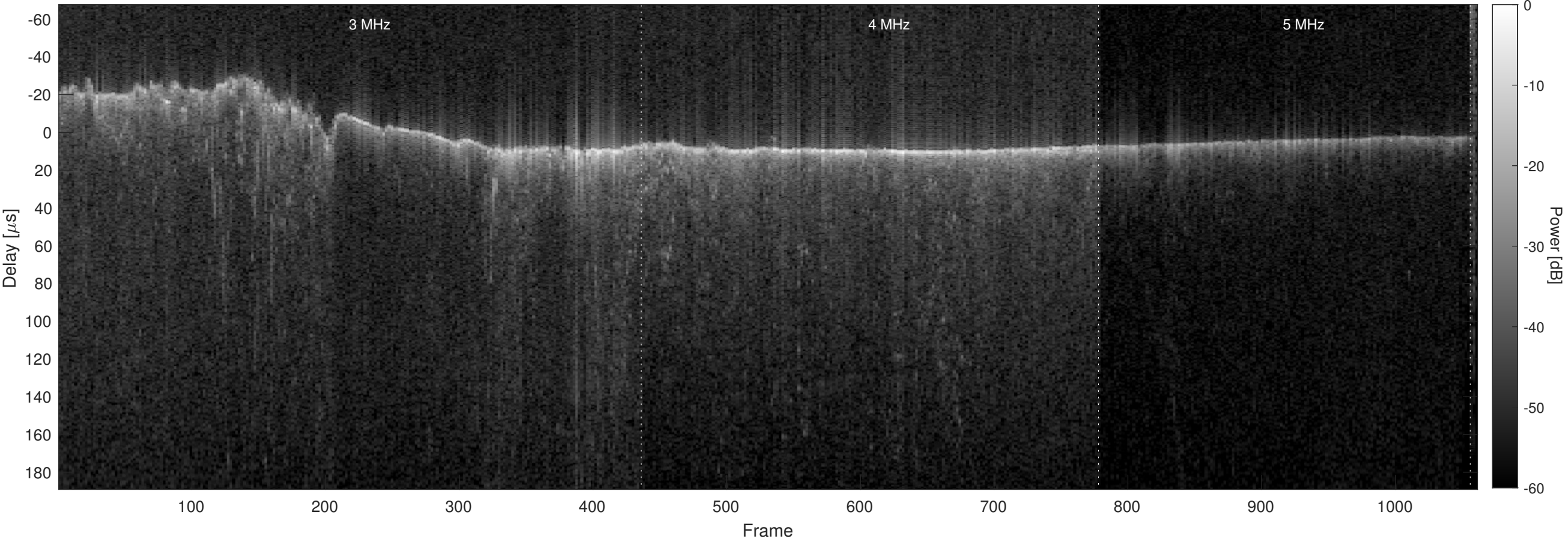
Orbit 8115, Optimized, No Window, Channel 2
