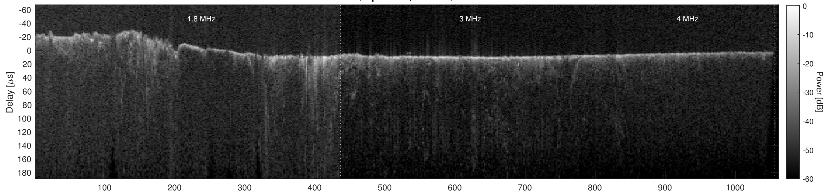
Orbit 8115, Cluttergram
