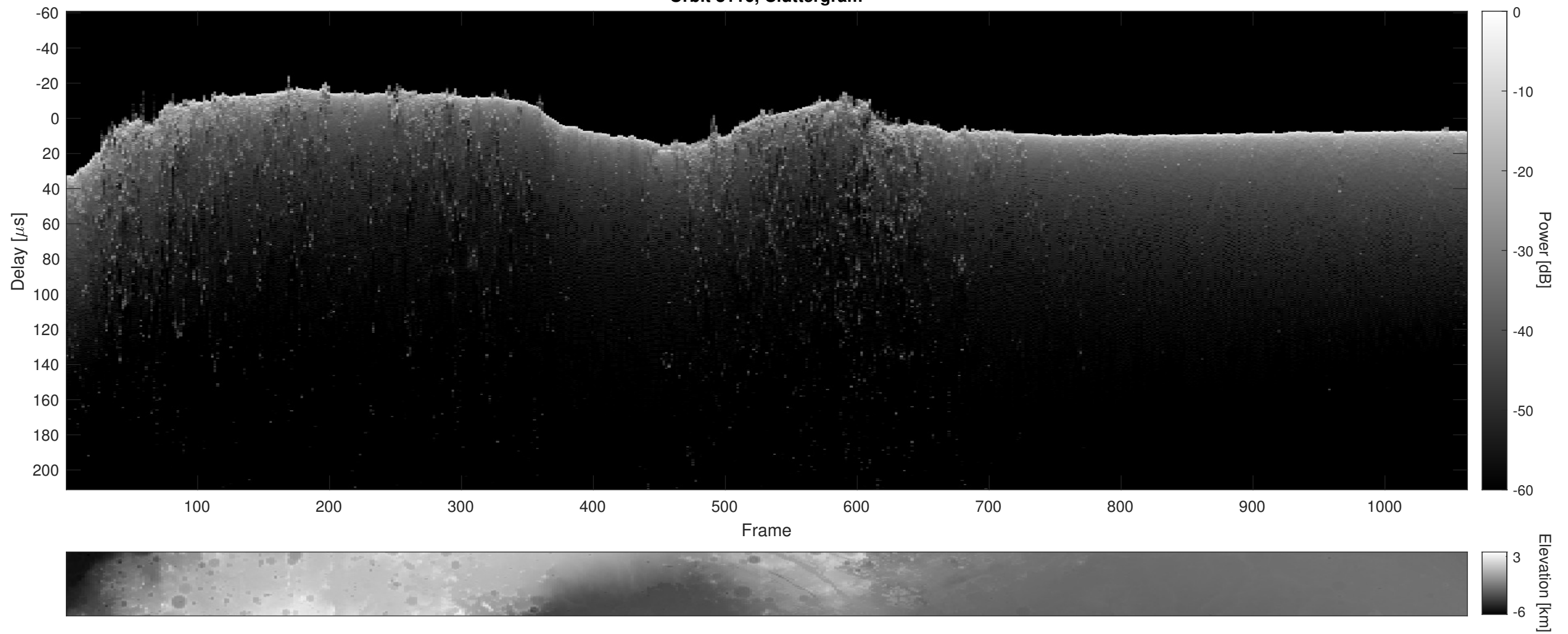
Orbit 8116, Cluttergram
