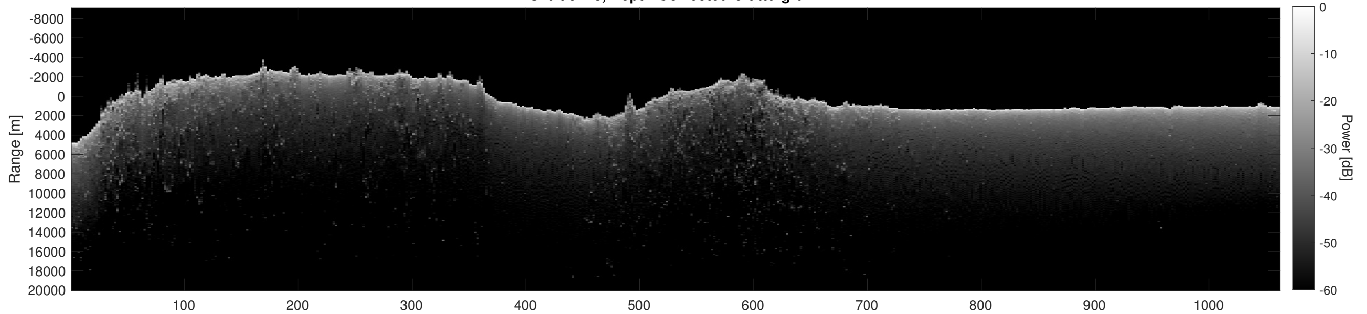
Orbit 8116, Depth-Corrected Cluttergram
