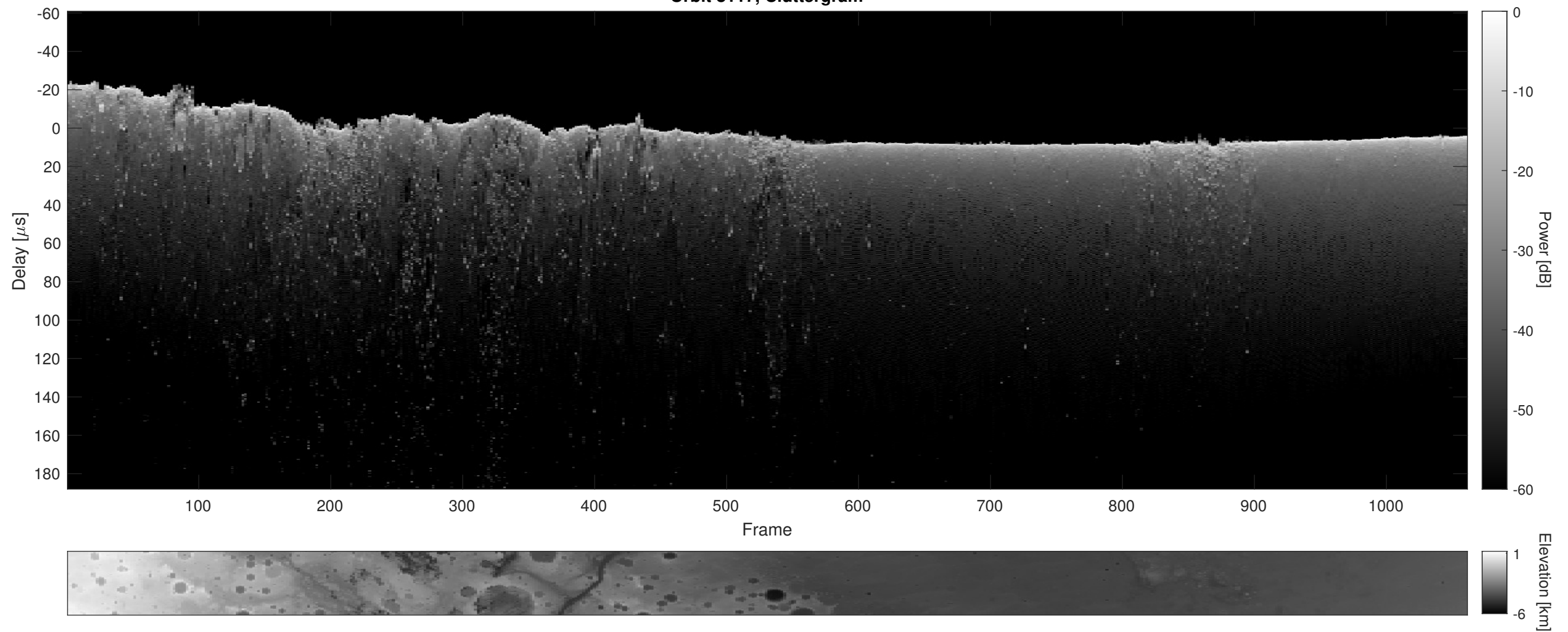
Orbit 8117, Cluttergram
