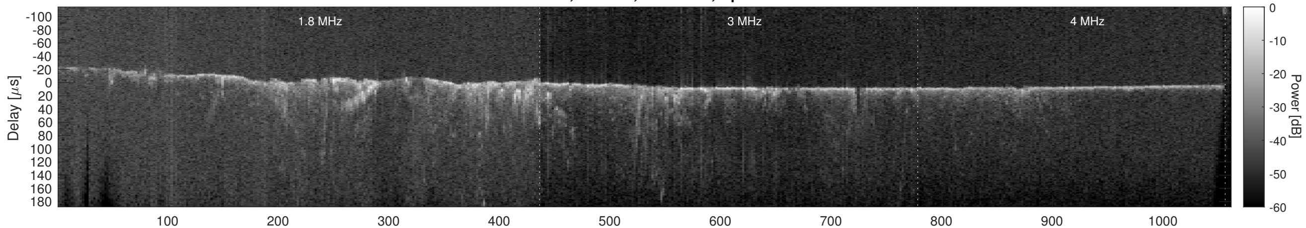
Orbit 8117, Cluttergram
