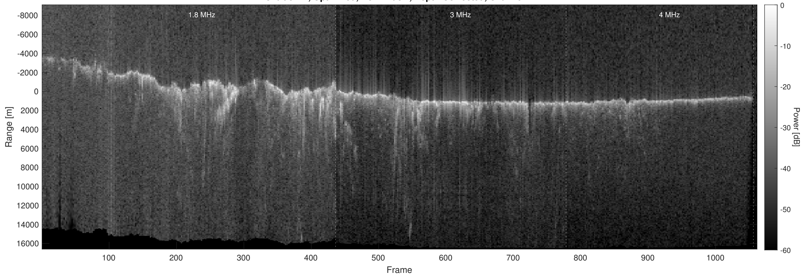
Orbit 8117, Optimized, No Window, Depth-Corrected, Channel 2
