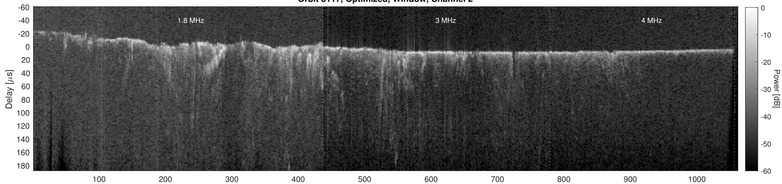
Orbit 8117, Cluttergram
