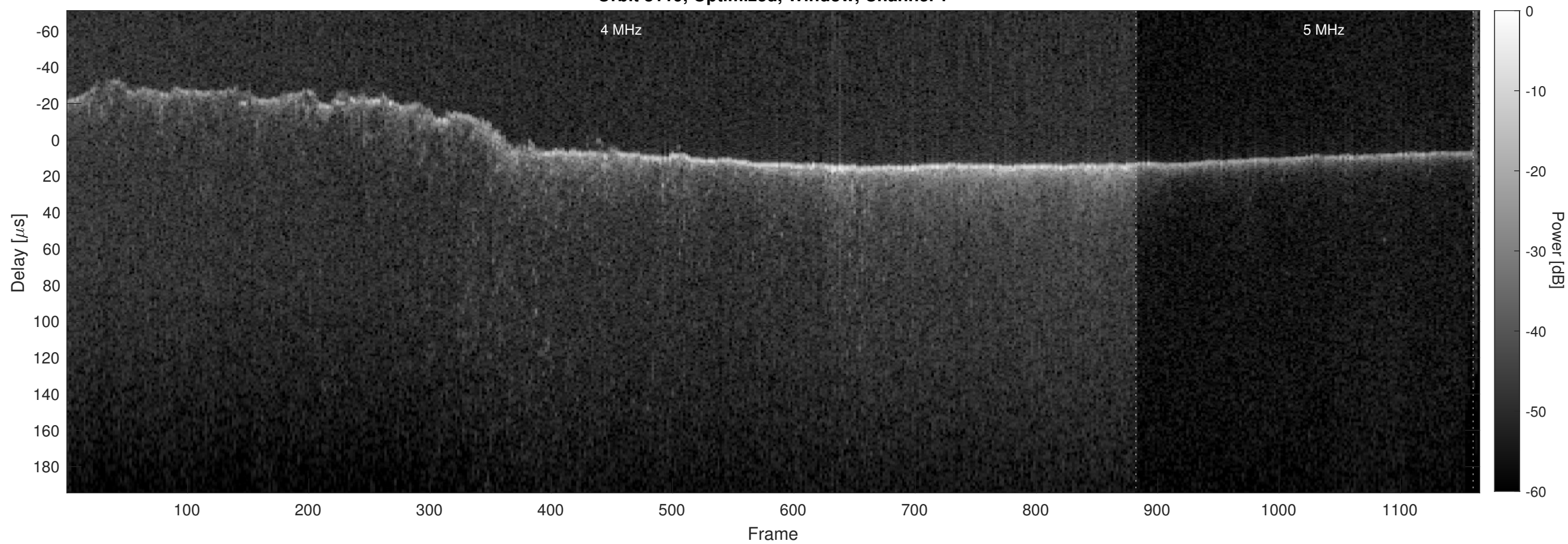
Orbit 8119, Optimized, Window, Channel 2
