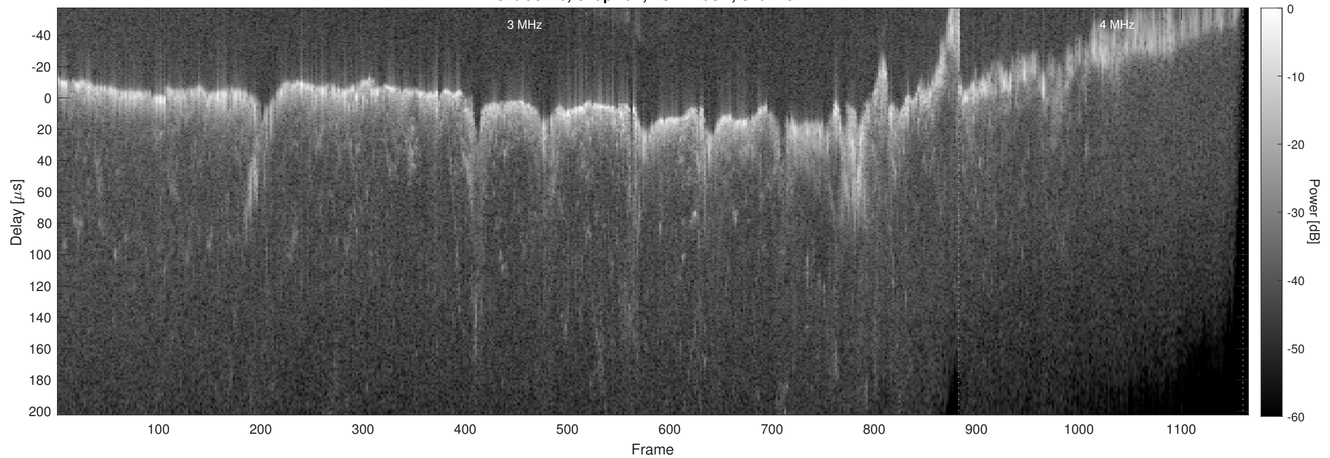
Orbit 8120, Chapman, No Window, Channel 2
