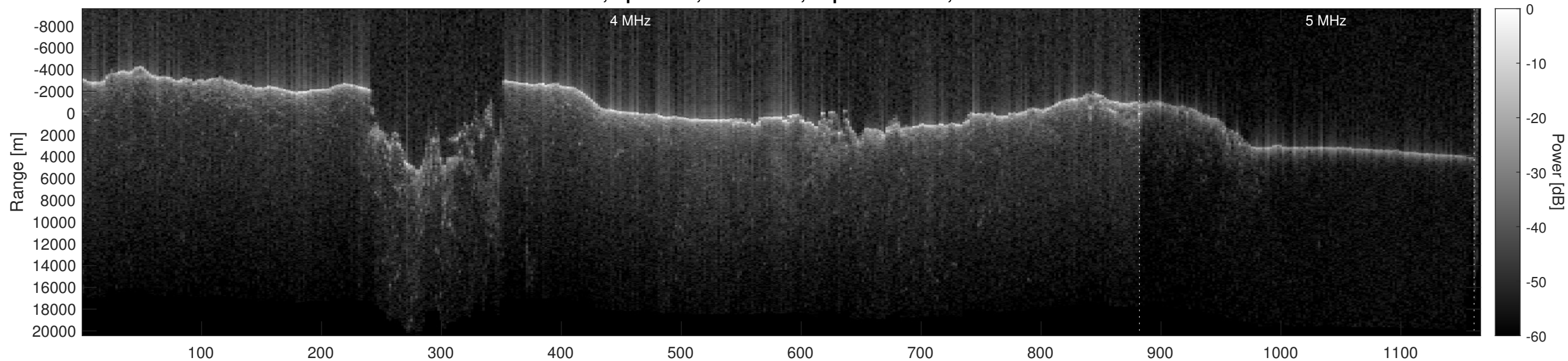
Orbit 8121, Optimized, No Window, Depth-Corrected, Channel 2
