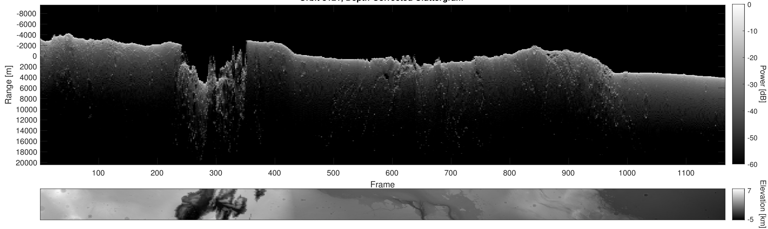
Orbit 8121, Depth-Corrected Cluttergram
