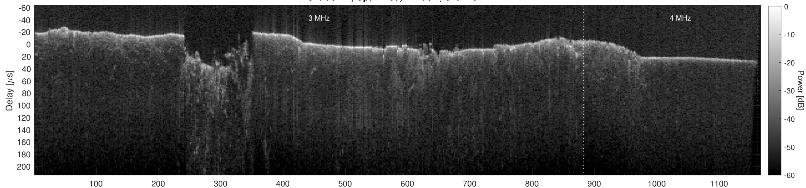
Orbit 8121, Cluttergram
