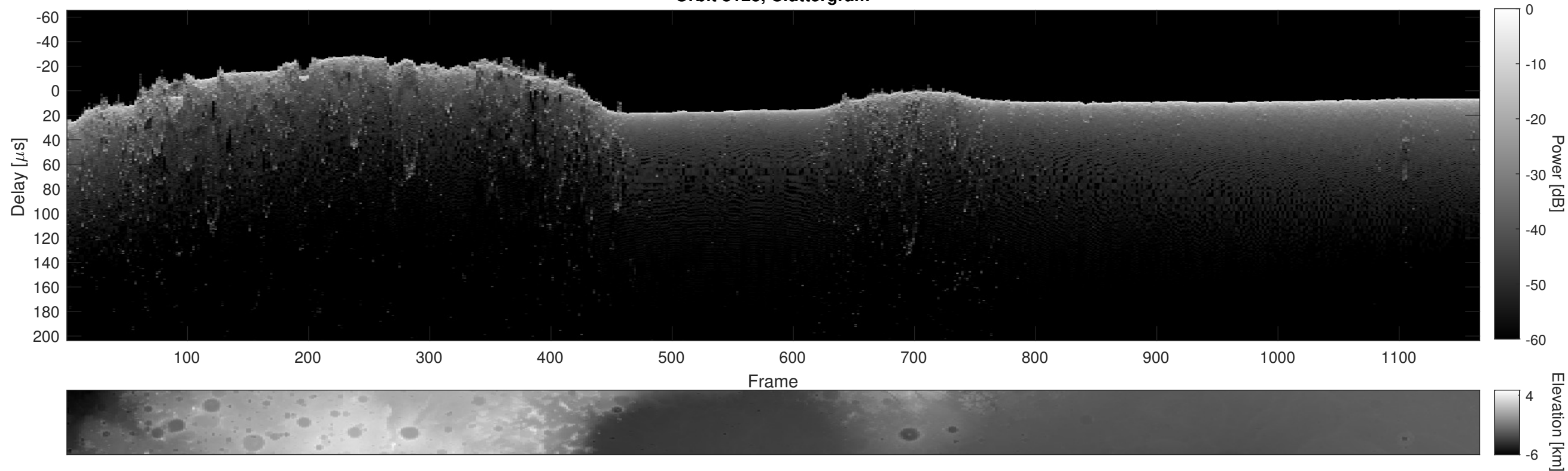
Orbit 8123, Cluttergram
