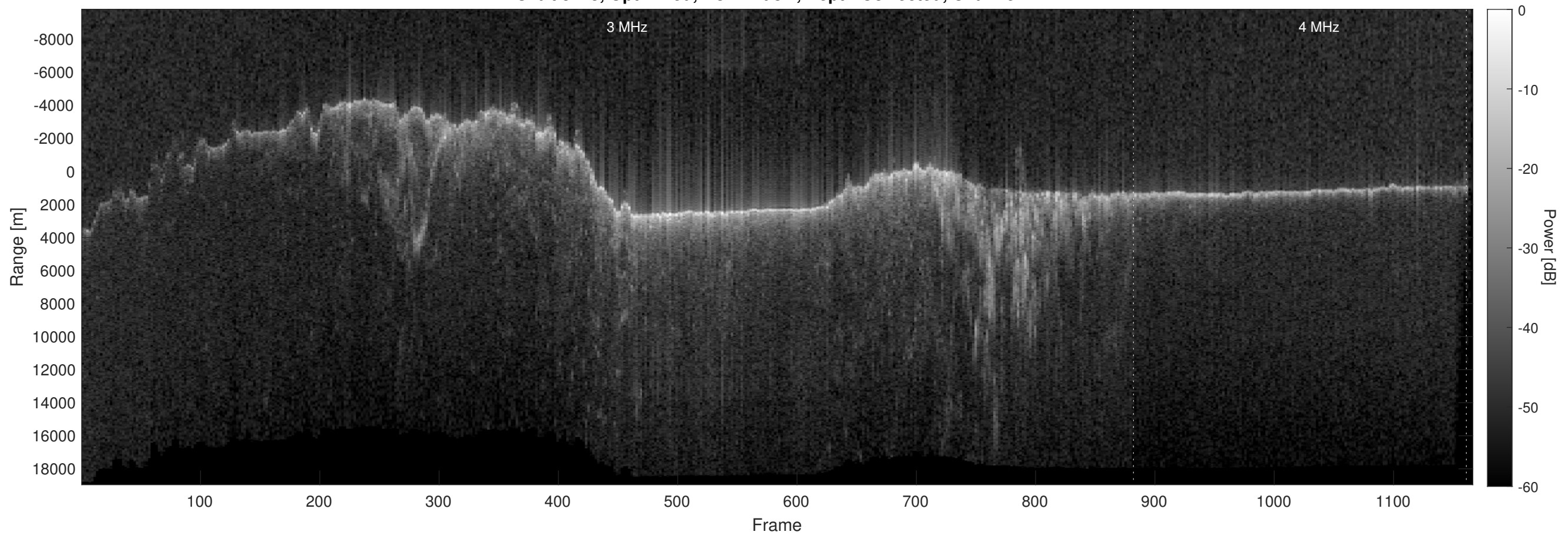
Orbit 8123, Optimized, No Window, Depth-Corrected, Channel 2
