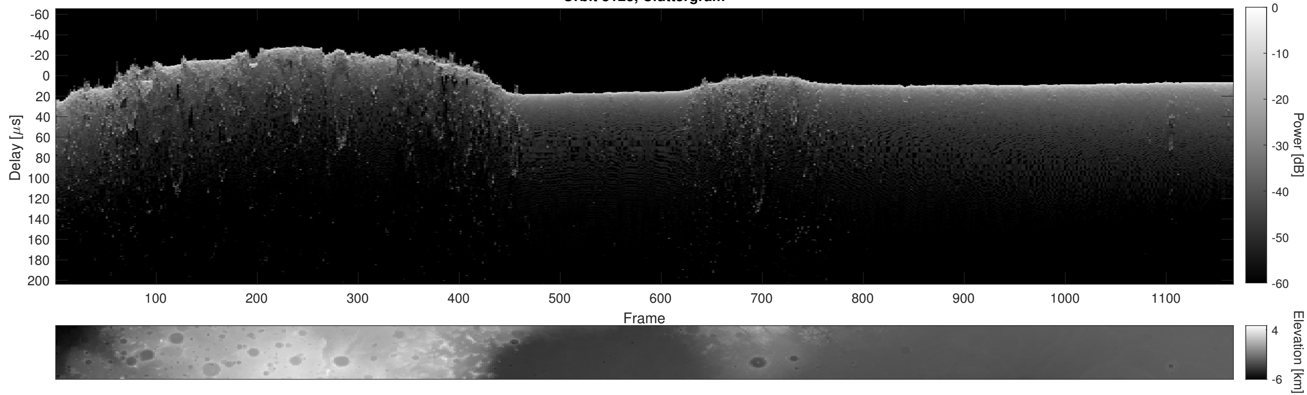
Orbit 8123, Cluttergram
