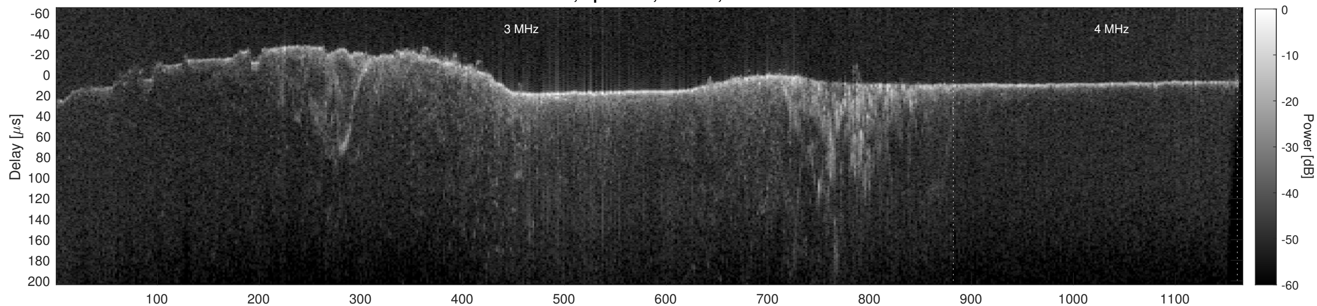
Orbit 8123, Cluttergram
