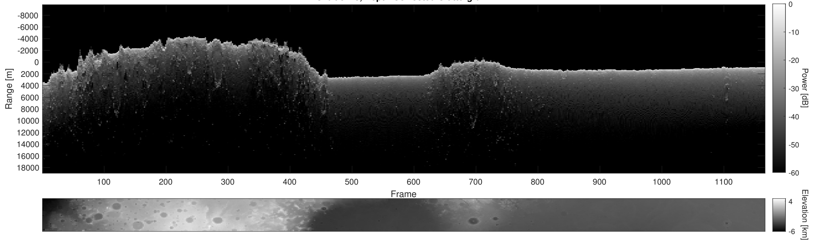
Orbit 8123, Depth-Corrected Cluttergram
