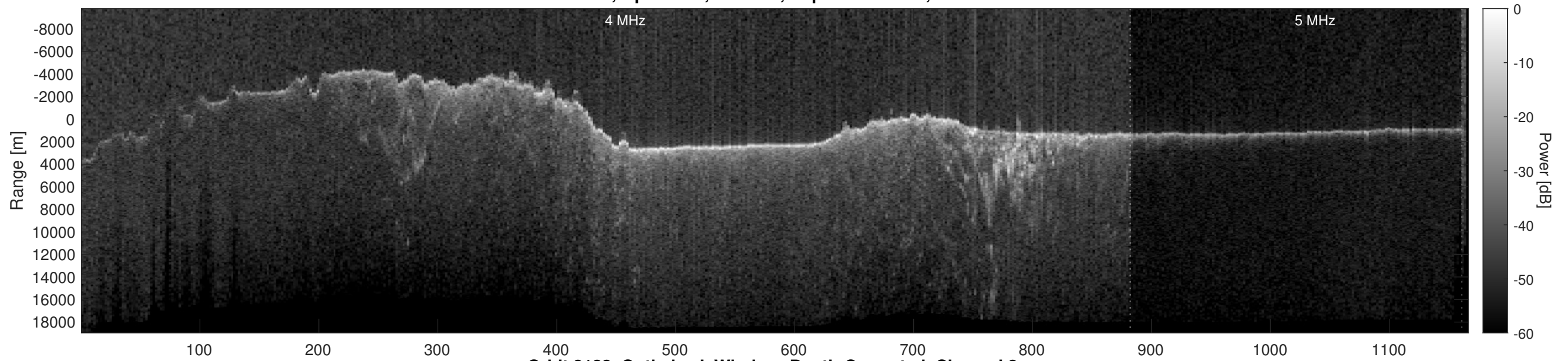
Orbit 8123, Optimized, Window, Depth-Corrected, Channel 2
