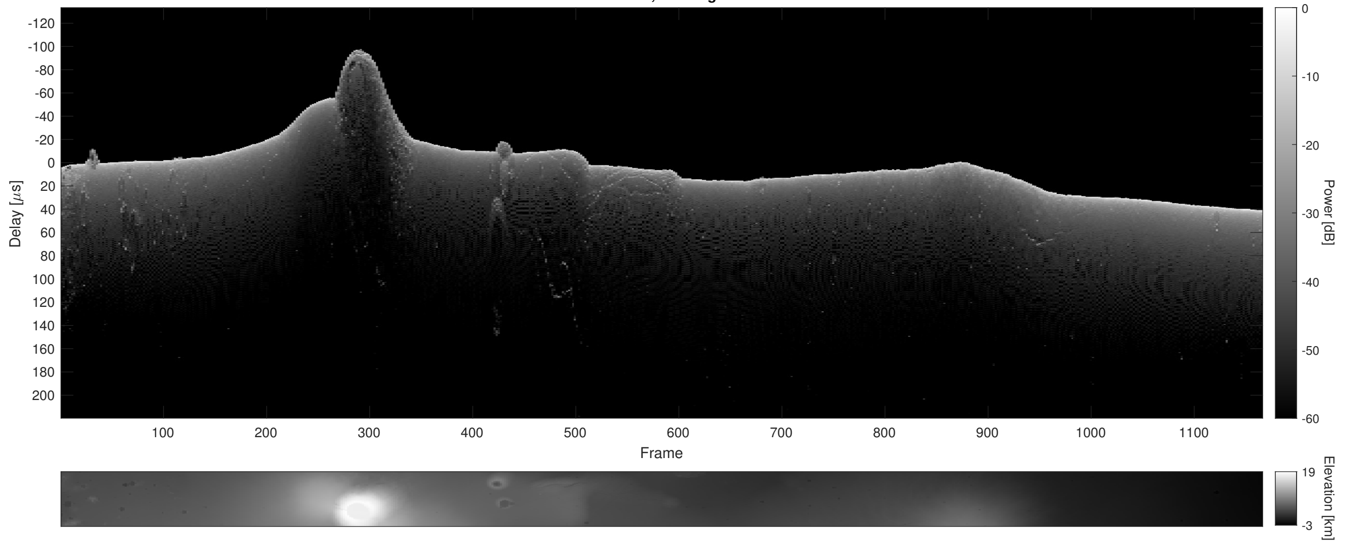
Orbit 8125, Cluttergram
