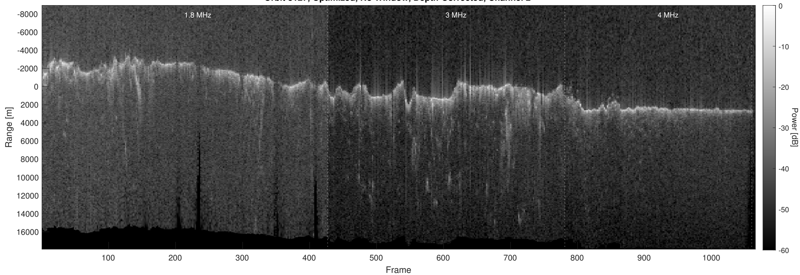
Orbit 8127, Optimized, No Window, Depth-Corrected, Channel 2
