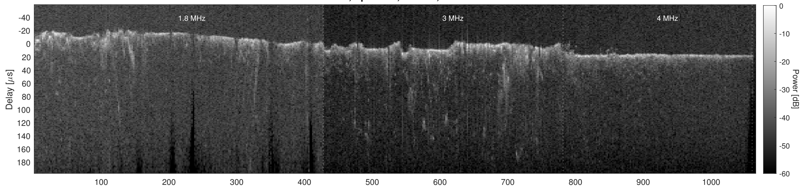
Orbit 8127, Cluttergram
