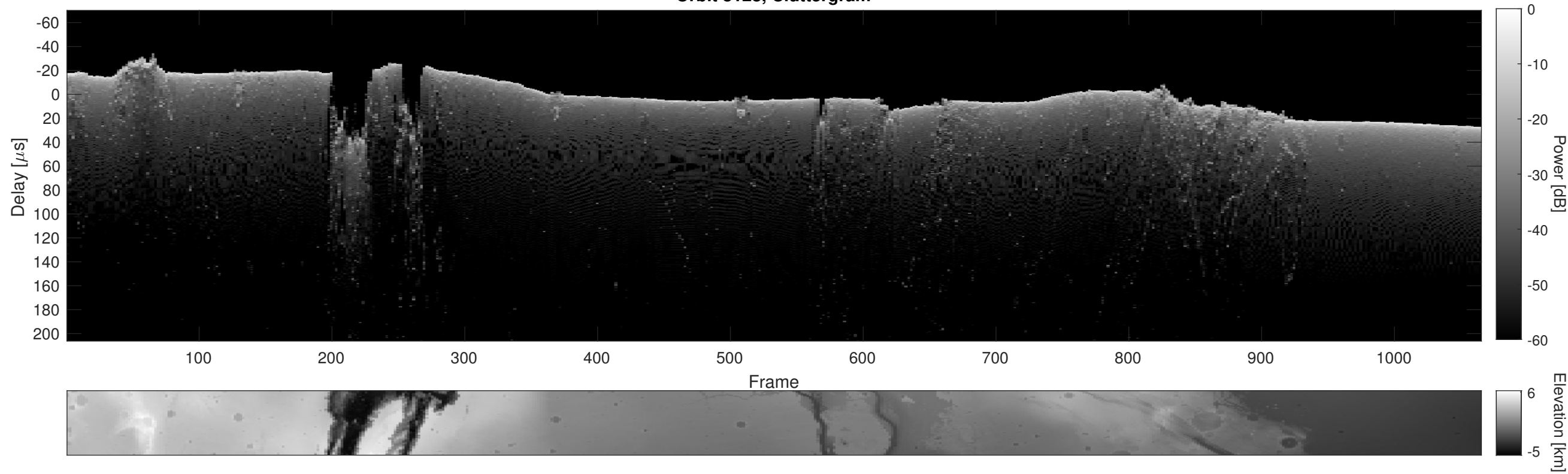
Orbit 8128, Cluttergram
