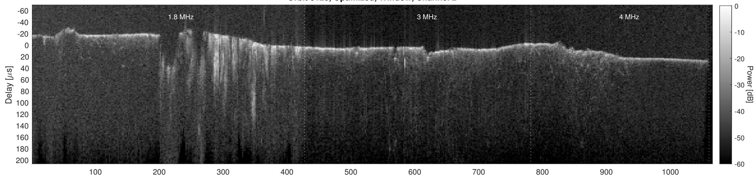
Orbit 8128, Cluttergram
