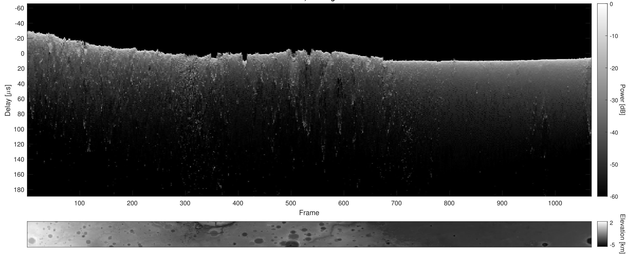
Orbit 8131, Cluttergram
