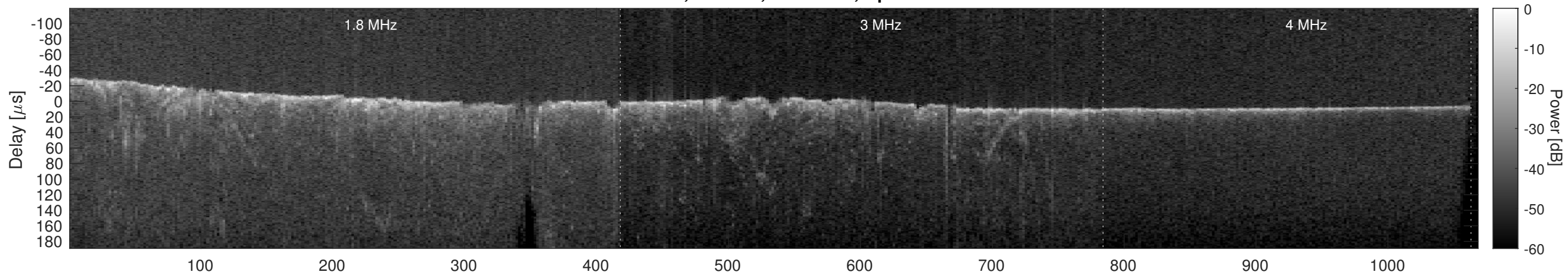
Orbit 8131, Cluttergram
