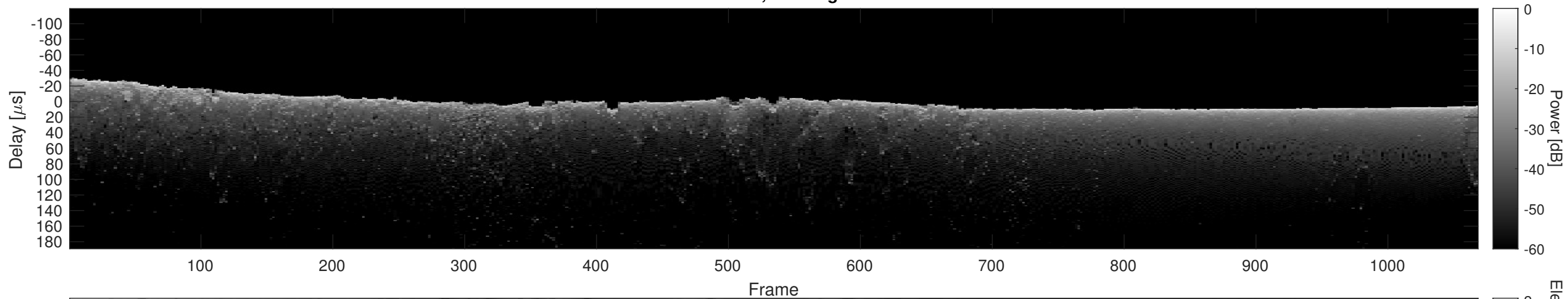
Orbit 8131, Cluttergram
