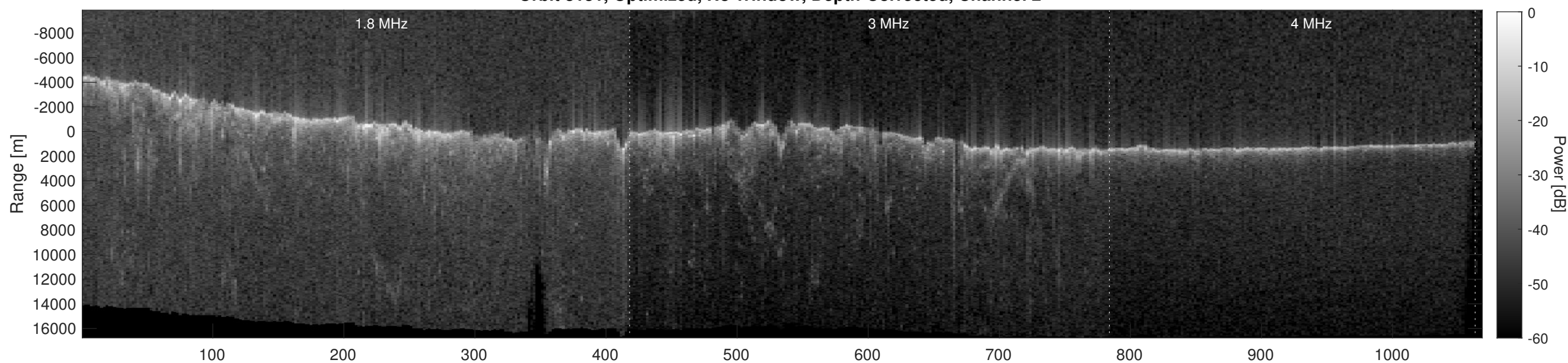
Orbit 8131, Depth-Corrected Cluttergram
