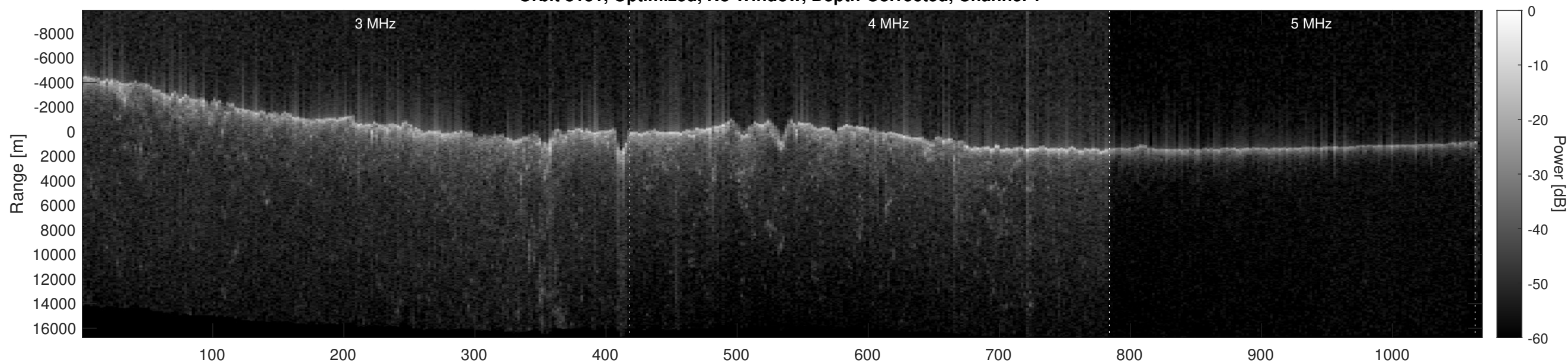
Orbit 8131, Optimized, No Window, Depth-Corrected, Channel 2
