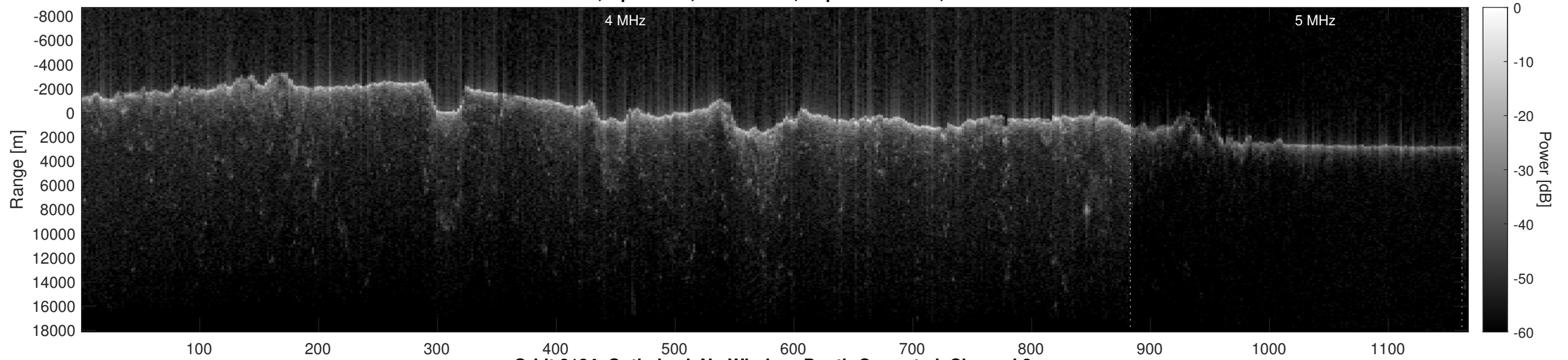
Orbit 8134, Optimized, No Window, Depth-Corrected, Channel 2
