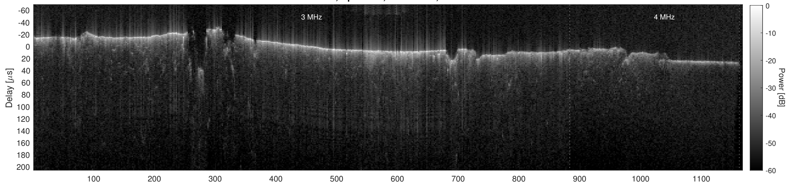
Orbit 8135, Cluttergram
