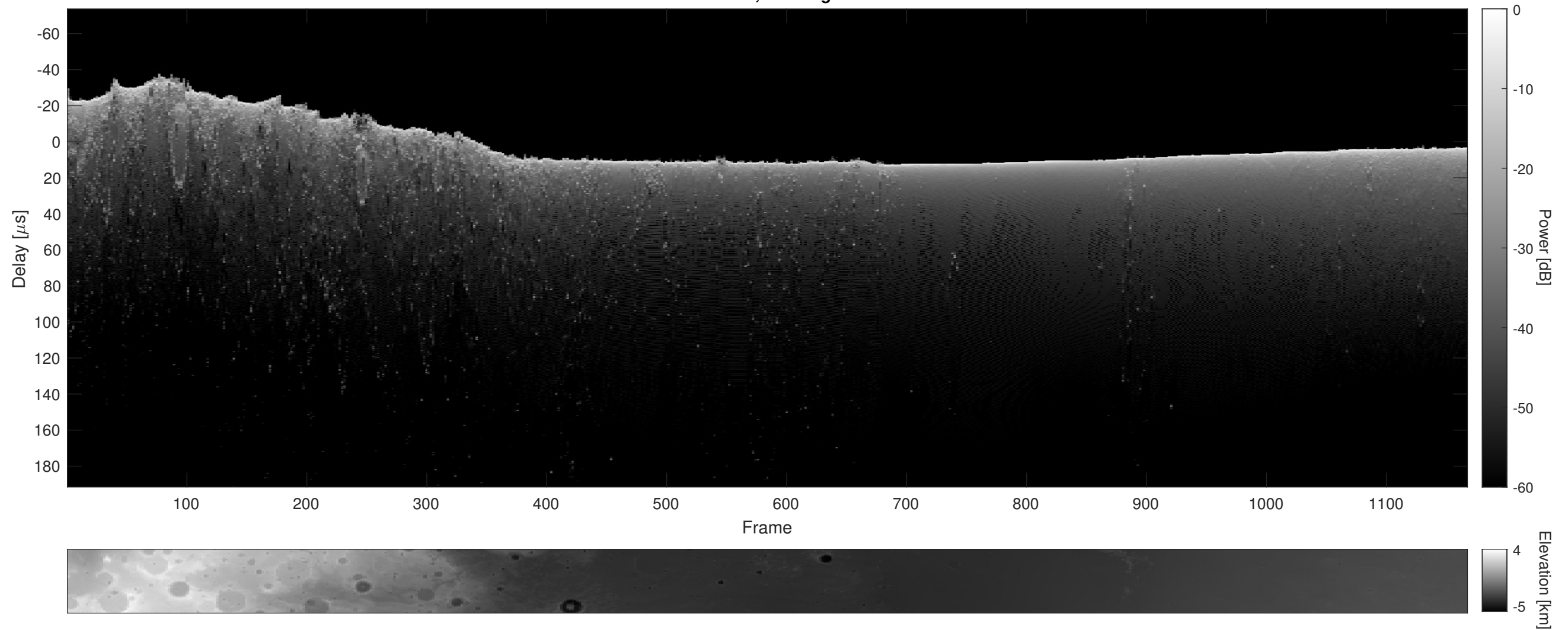
Orbit 8136, Cluttergram
