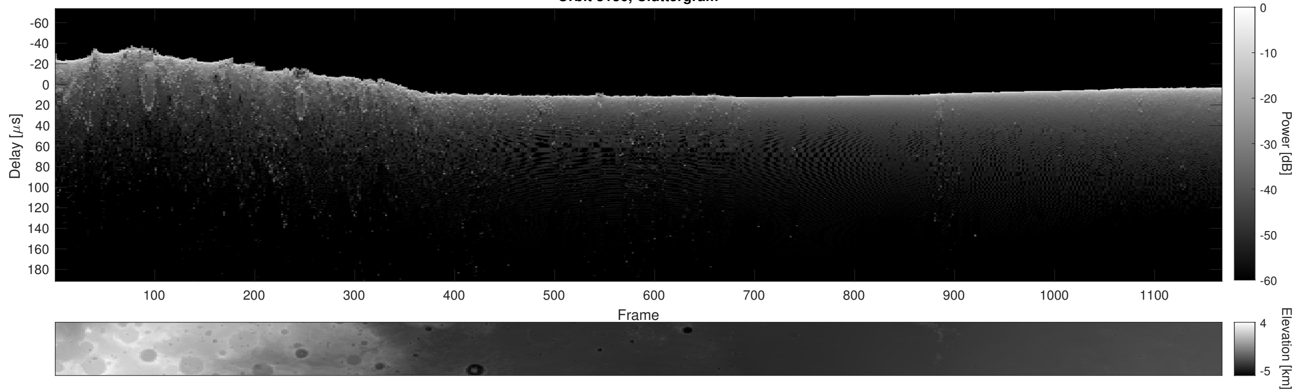
Orbit 8136, Cluttergram
