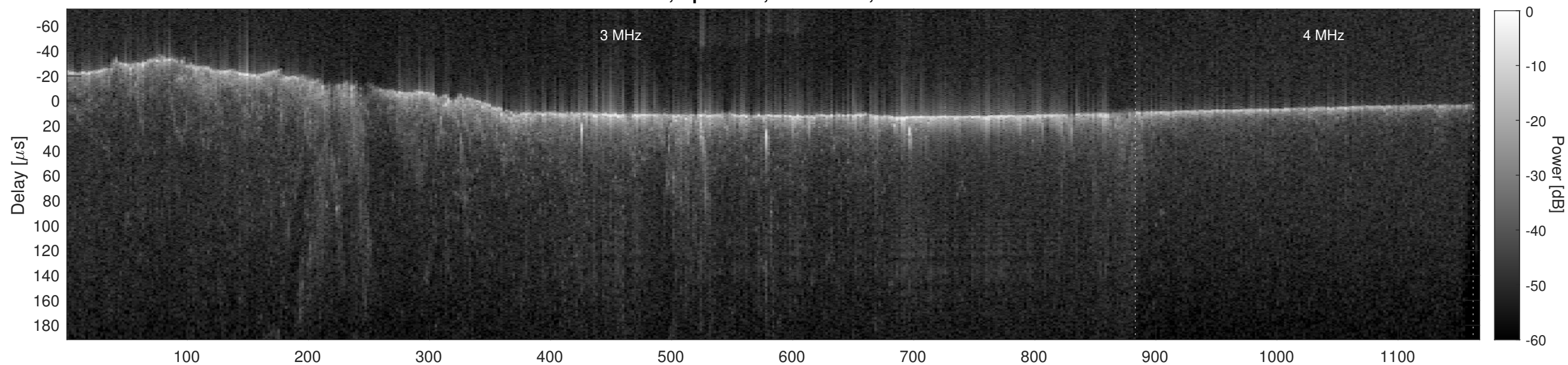
Orbit 8136, Cluttergram
