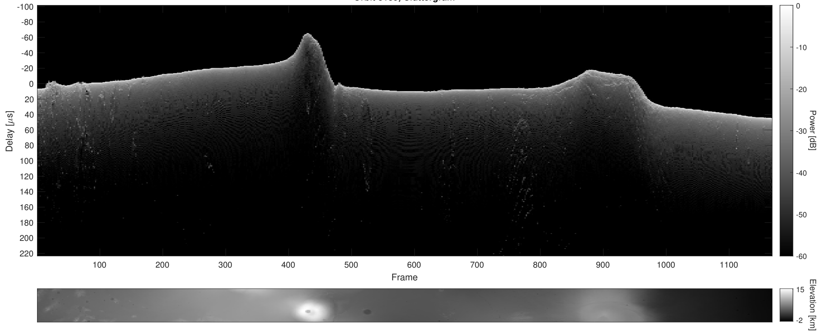
Orbit 8139, Cluttergram
