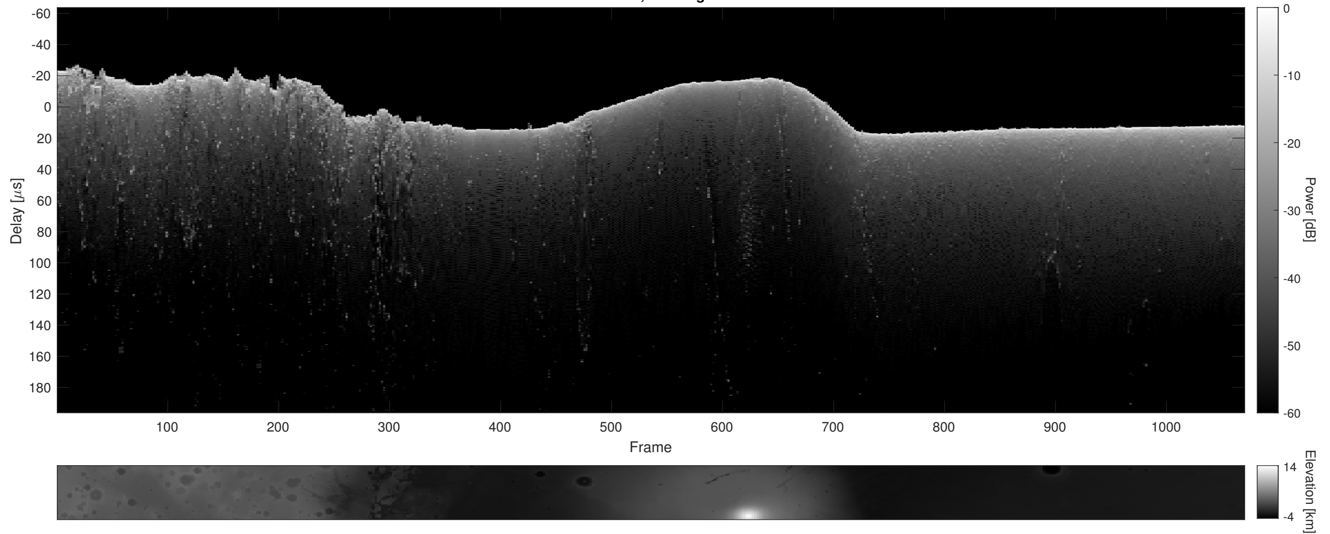
Orbit 8140, Cluttergram
