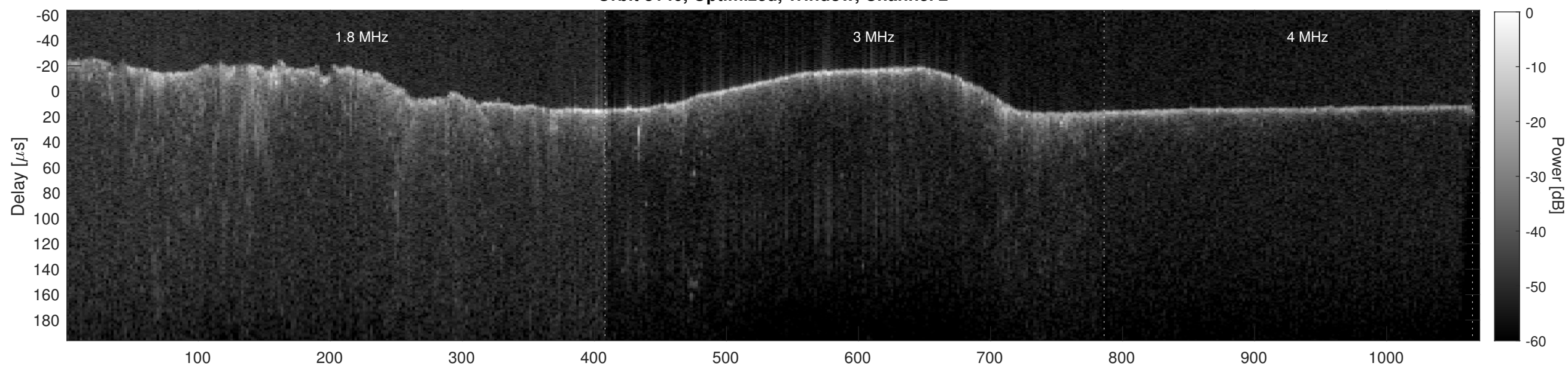
Orbit 8140, Cluttergram
