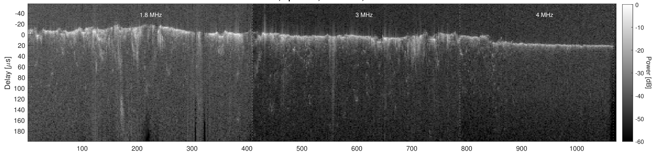
Orbit 8141, Cluttergram
