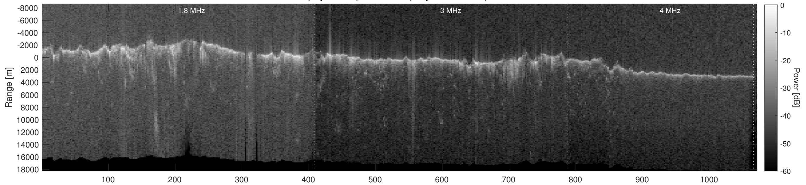
Orbit 8141, Depth-Corrected Cluttergram
