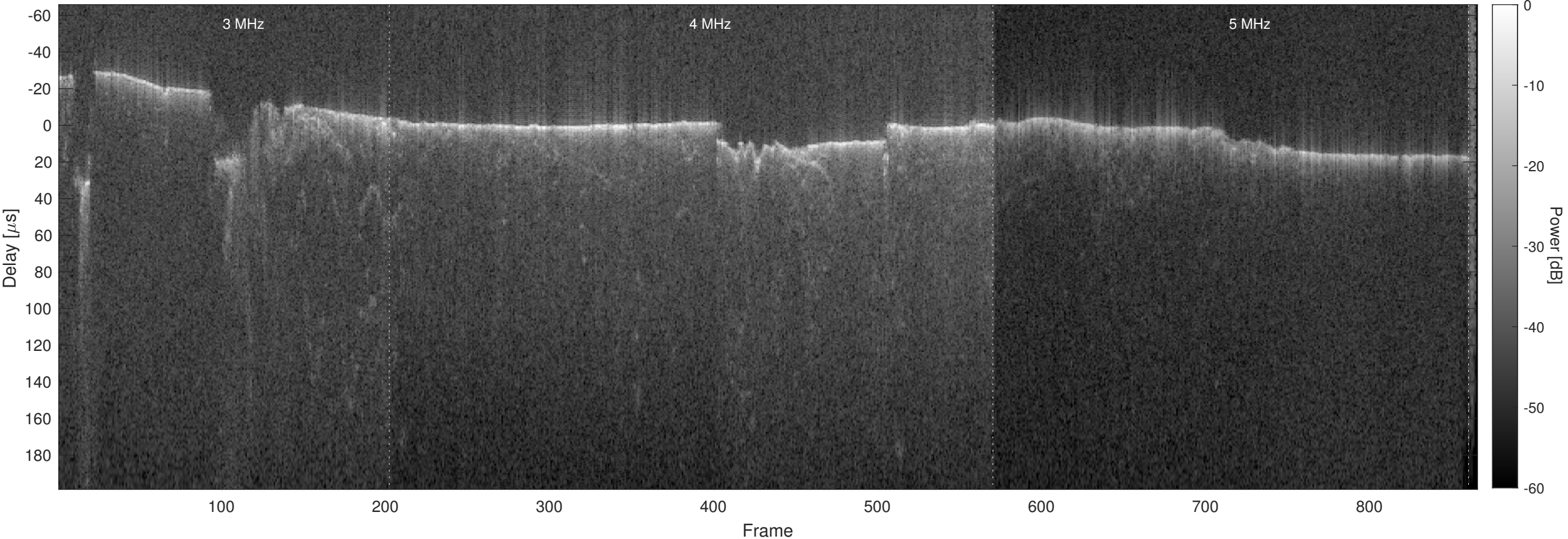
Orbit 8142, Optimized, No Window, Channel 2
