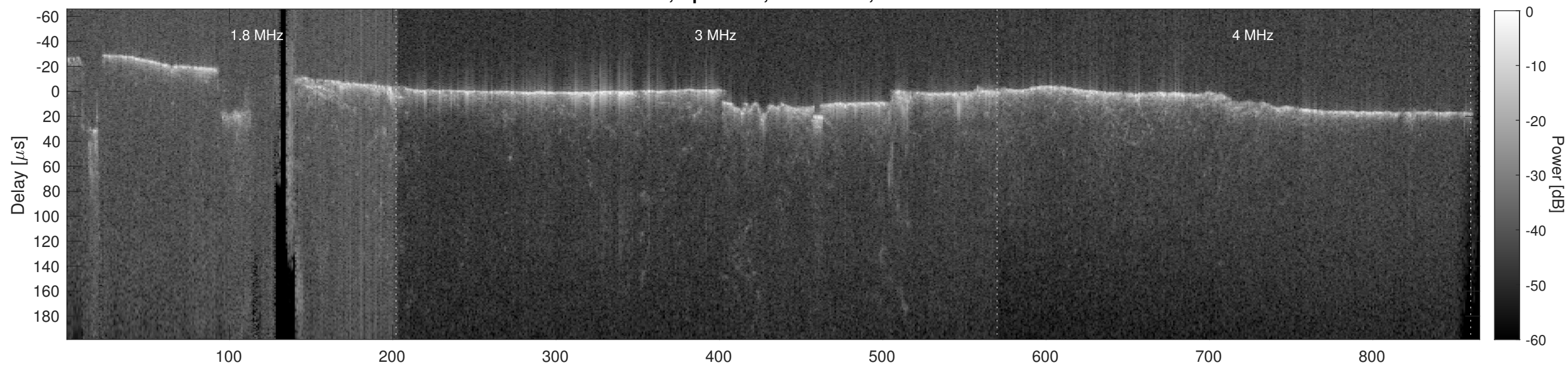
Orbit 8142, Cluttergram
