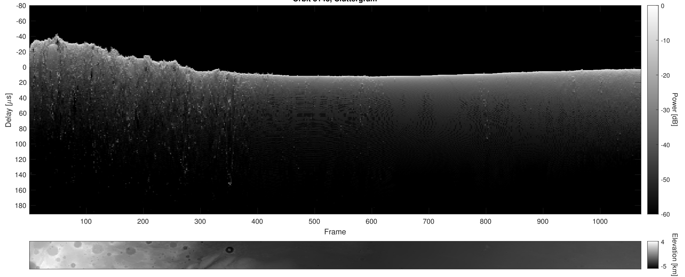
Orbit 8143, Cluttergram
