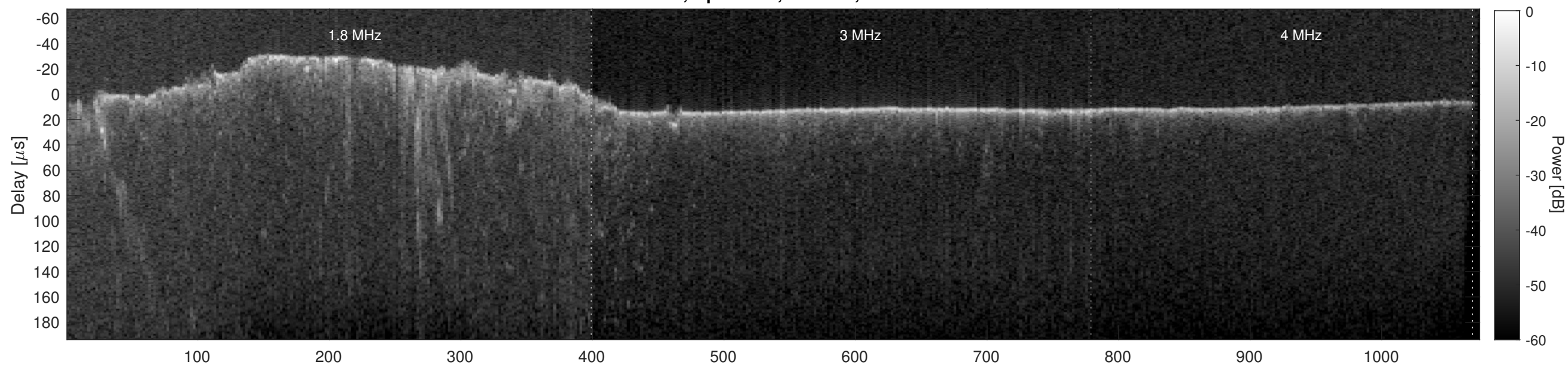
Orbit 8144, Cluttergram
