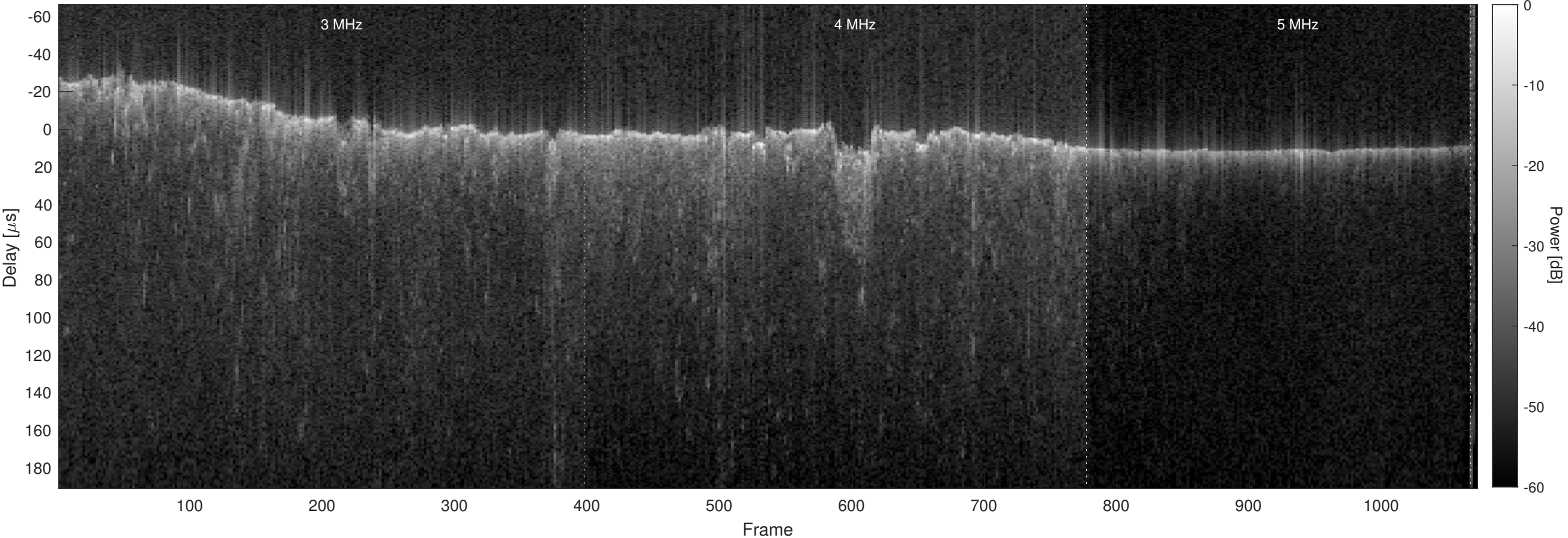
Orbit 8145, Optimized, No Window, Channel 2
