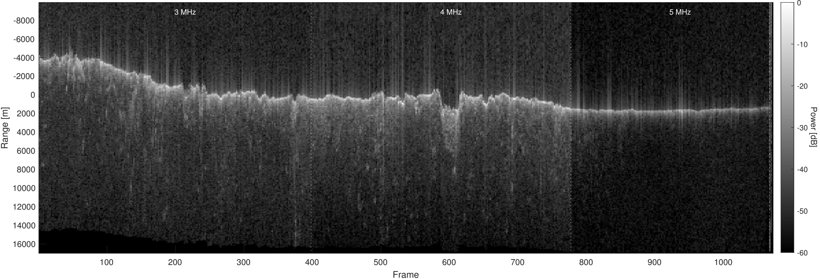
Orbit 8145, Optimized, No Window, Depth-Corrected, Channel 2
