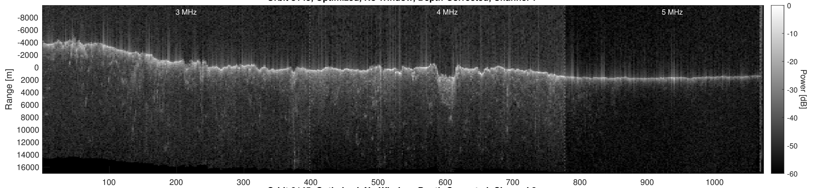
Orbit 8145, Optimized, No Window, Depth-Corrected, Channel 2
