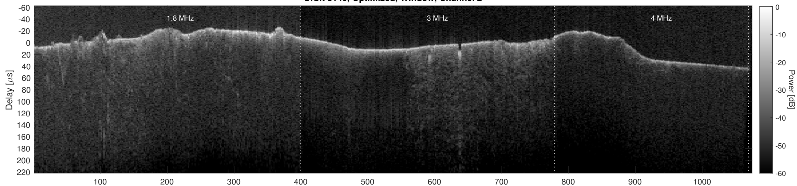
Orbit 8146, Cluttergram
