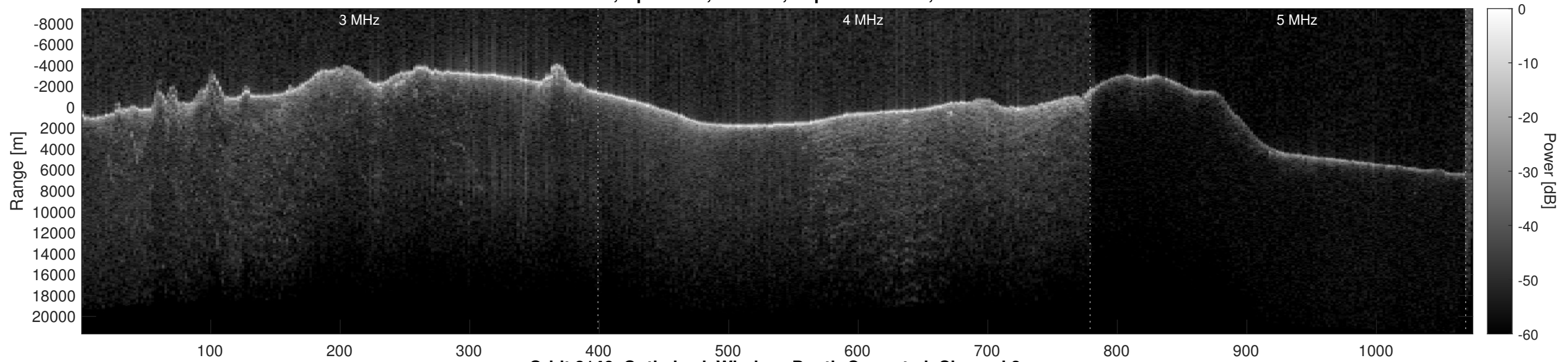
Orbit 8146, Optimized, Window, Depth-Corrected, Channel 2
