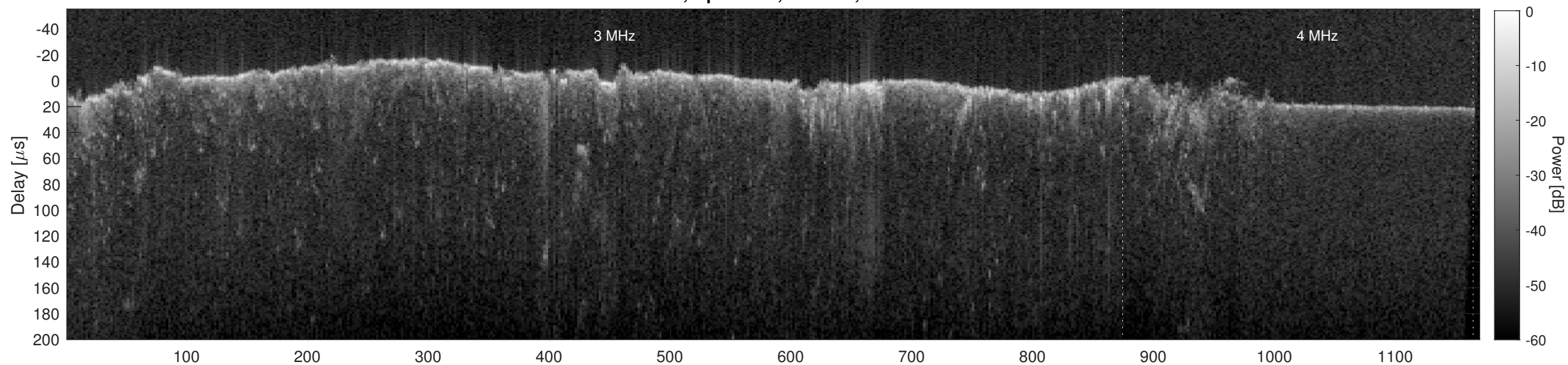
Orbit 8148, Cluttergram
