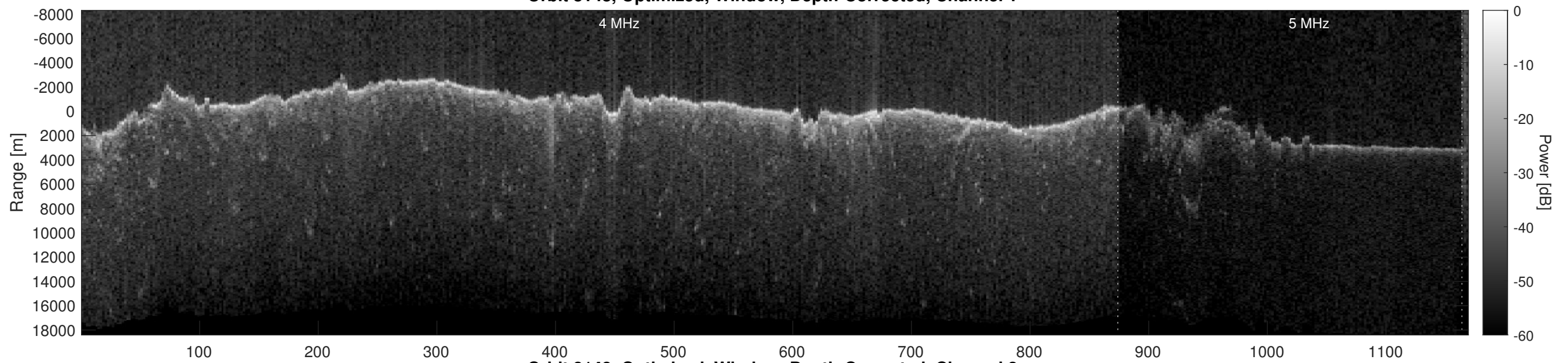
Orbit 8148, Optimized, Window, Depth-Corrected, Channel 2
