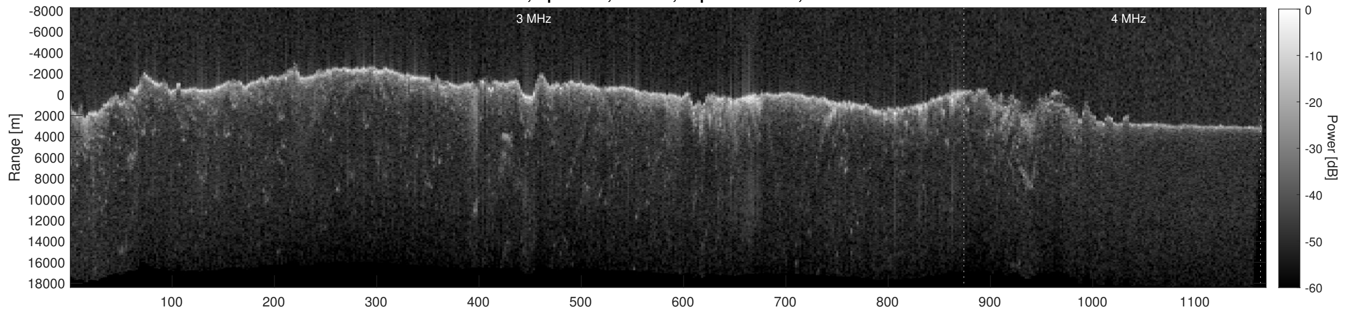
Orbit 8148, Depth-Corrected Cluttergram
