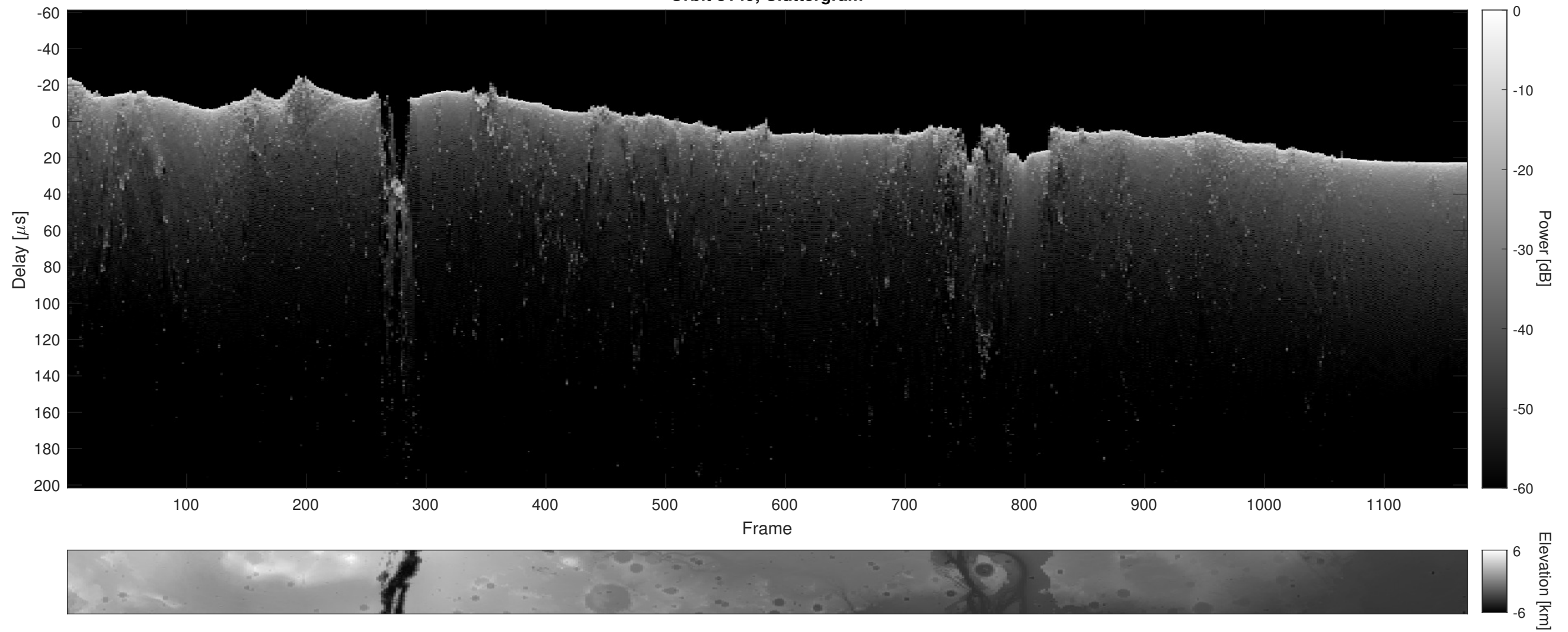
Orbit 8149, Cluttergram
