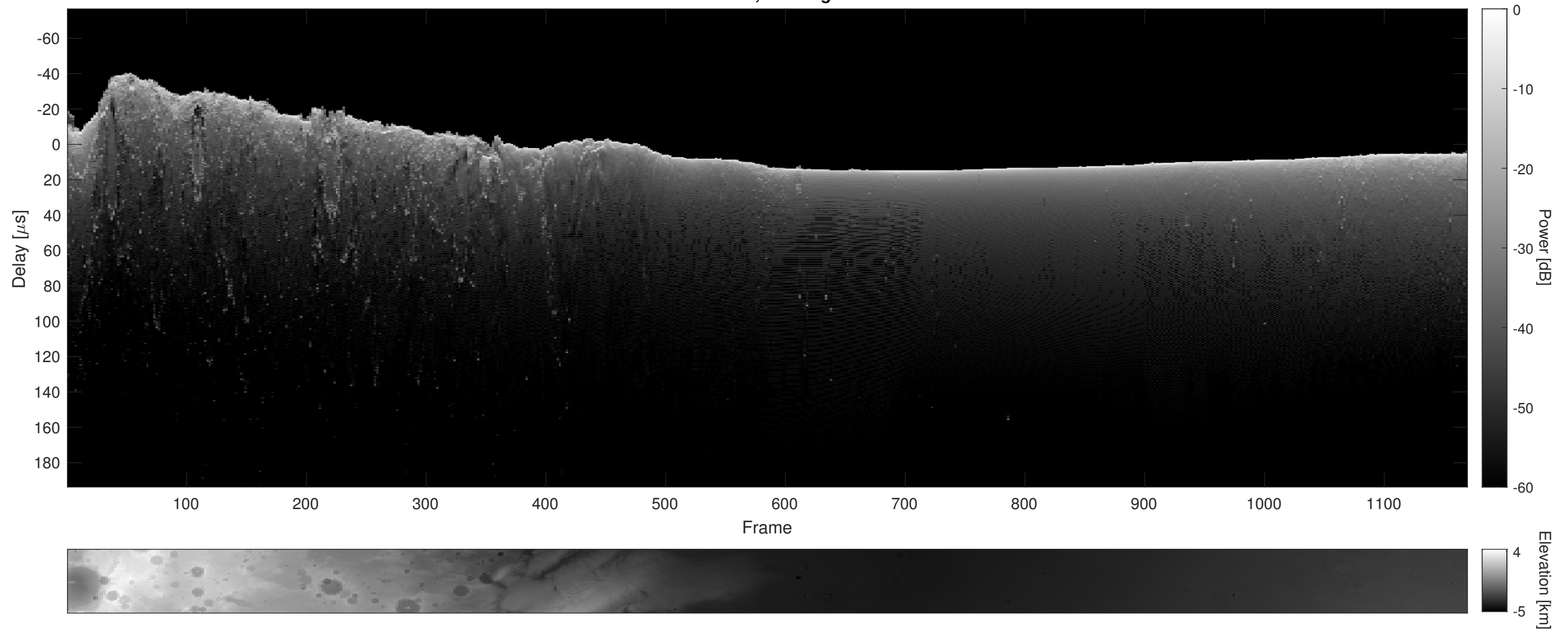
Orbit 8150, Cluttergram
