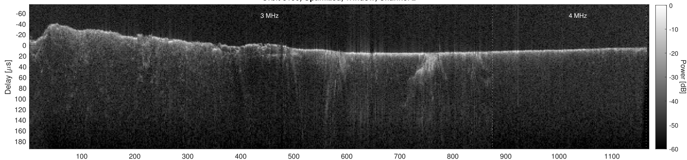
Orbit 8150, Cluttergram
