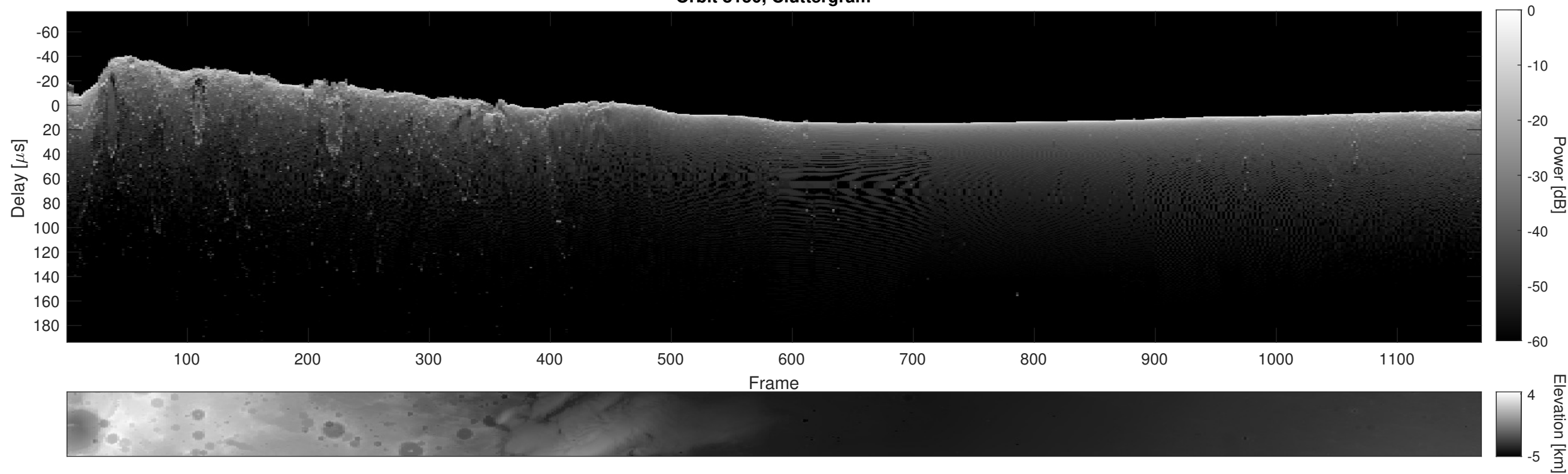
Orbit 8150, Cluttergram
