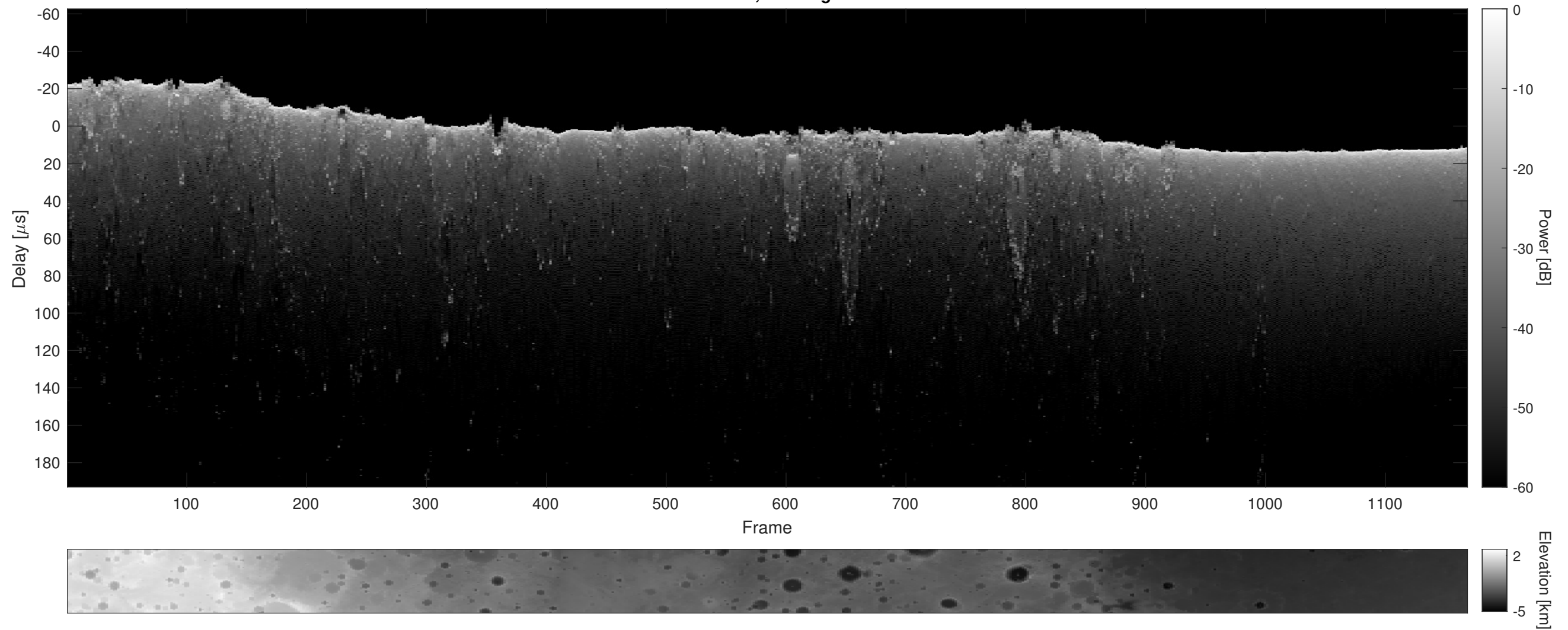
Orbit 8152, Cluttergram
