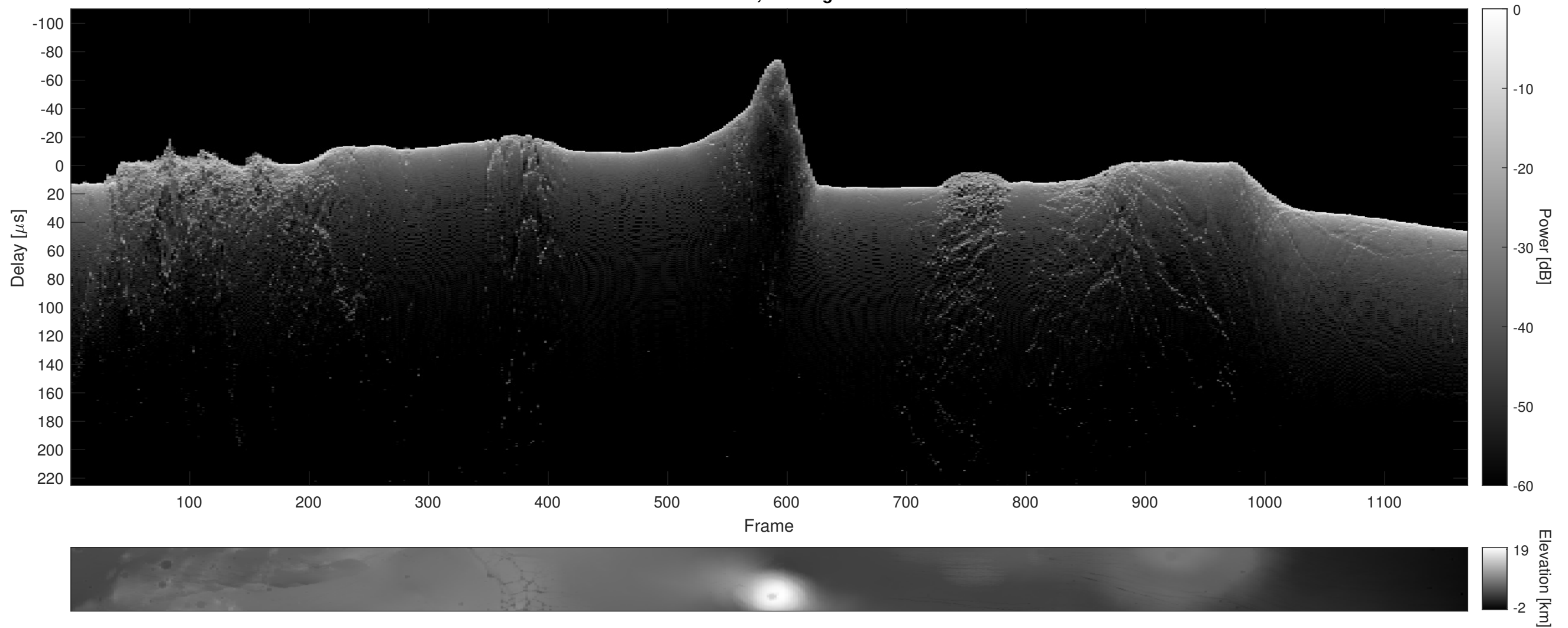
Orbit 8153, Cluttergram
