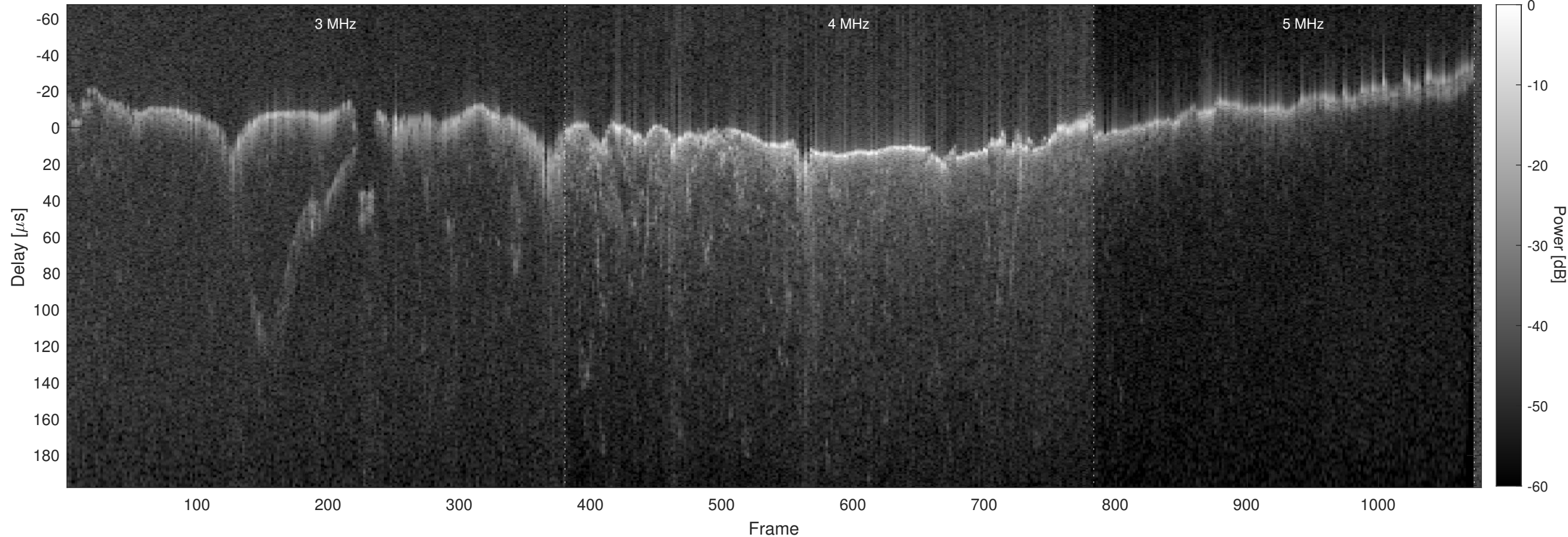
Orbit 8156, Chapman, No Window, Channel 2
